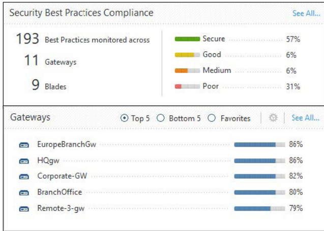
Security Overview
