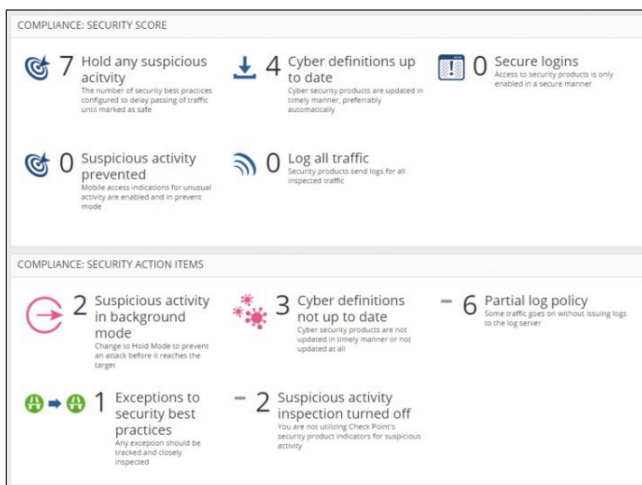
Security Violations
