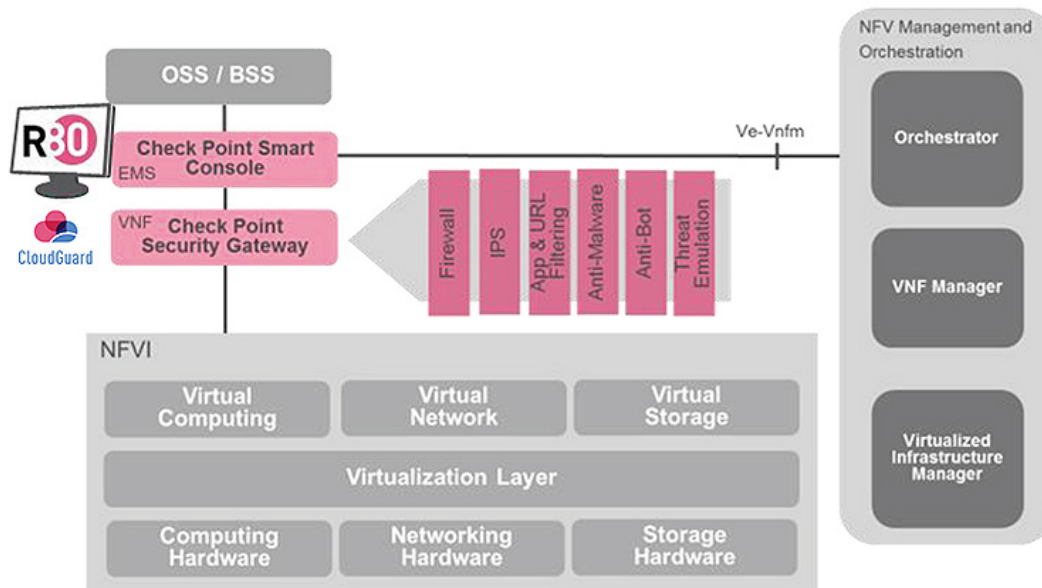
Check Point CloudGuard for OpenStack Integration with NFV infrastructure
